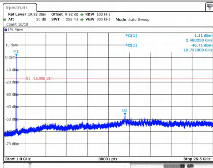
3DH5_Ant1_2480_1000~26500
