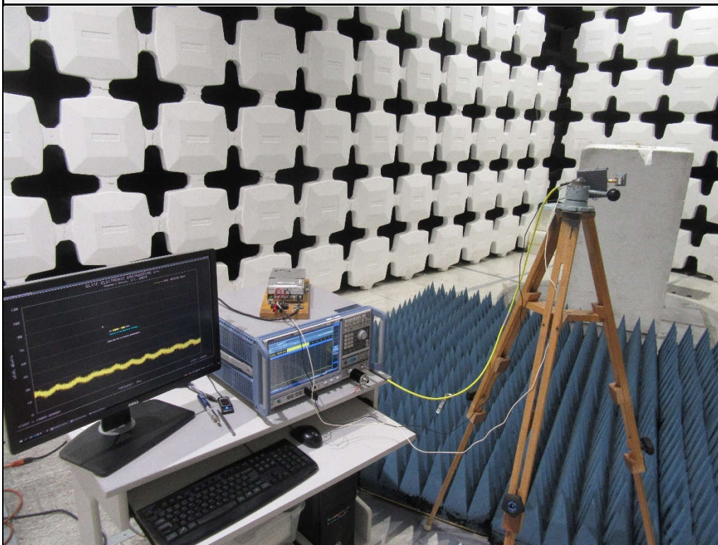
Test Setup for Spurious Radiated Emissions, 18GHz to 25GHz – Full Setup
