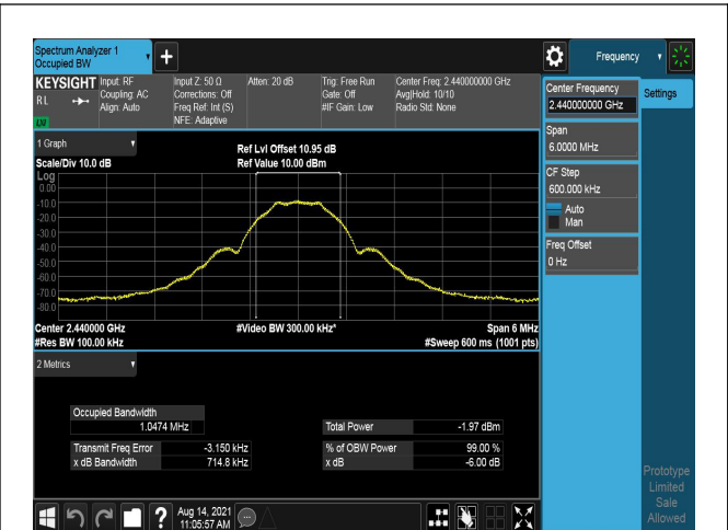
Modulation: Coded 125K 2440MHz
