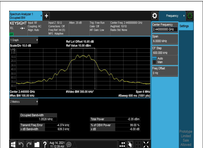
Modulation: Coded 500K 2440MHz
