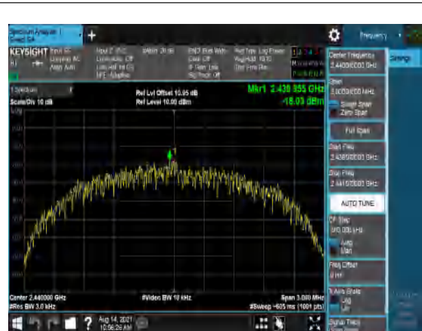
Modulation: 2Mbps 2440MHz
