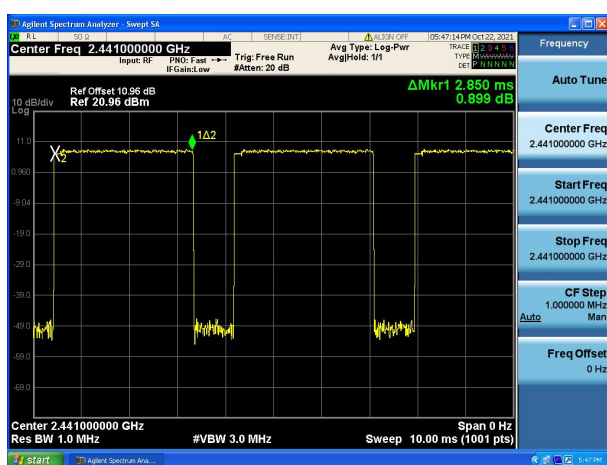
Modulation: \pi/4 DQPSK 2DH5 2441MHz
