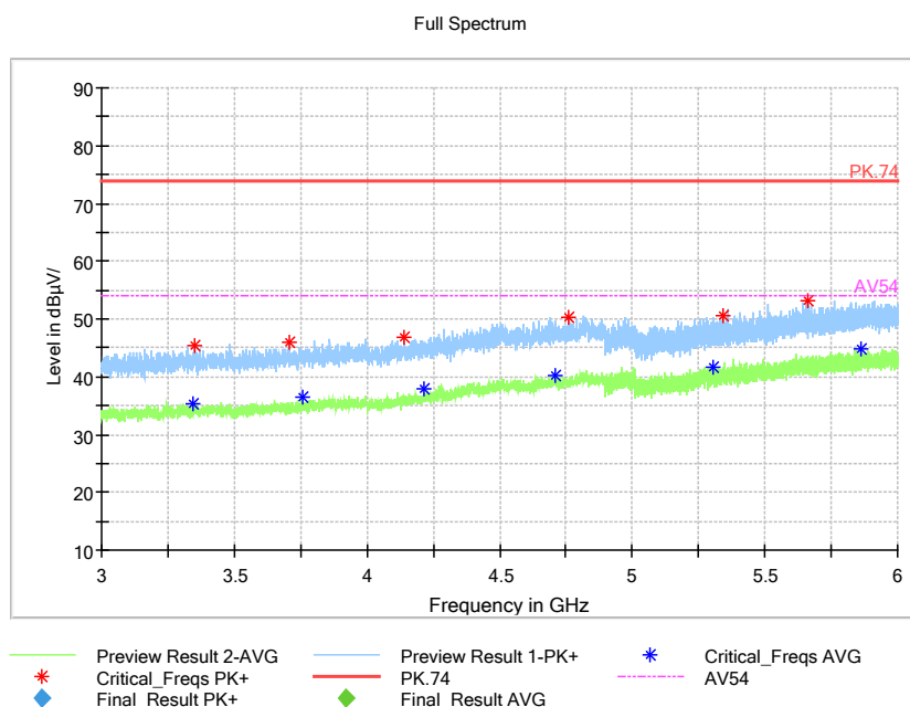
Pic12. Radiated emission (3GHz –6GHz)
