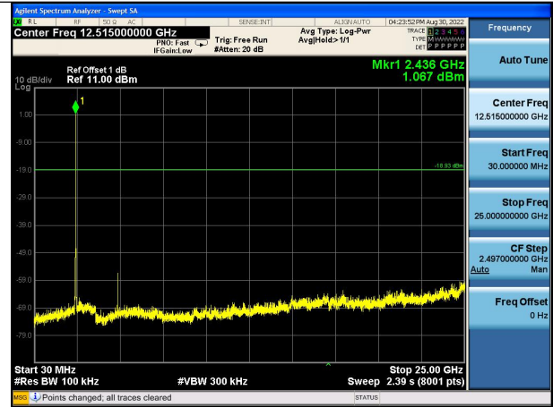
Test Mode:802.11b 2437MHz Chain0
