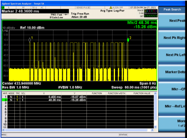
(Total Bursts in a transmit cycle 25pcs)
