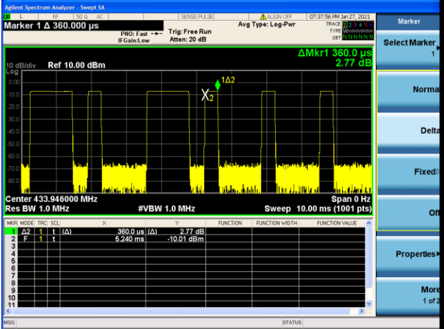
(Time per burst: 0.360ms*18pcs)
