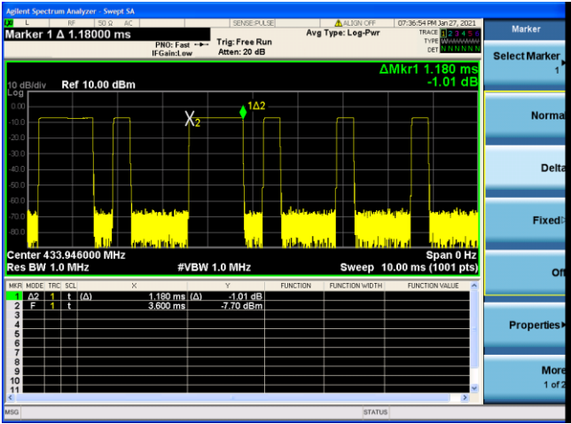
(Time per burst: 1.180ms*7pcs)
