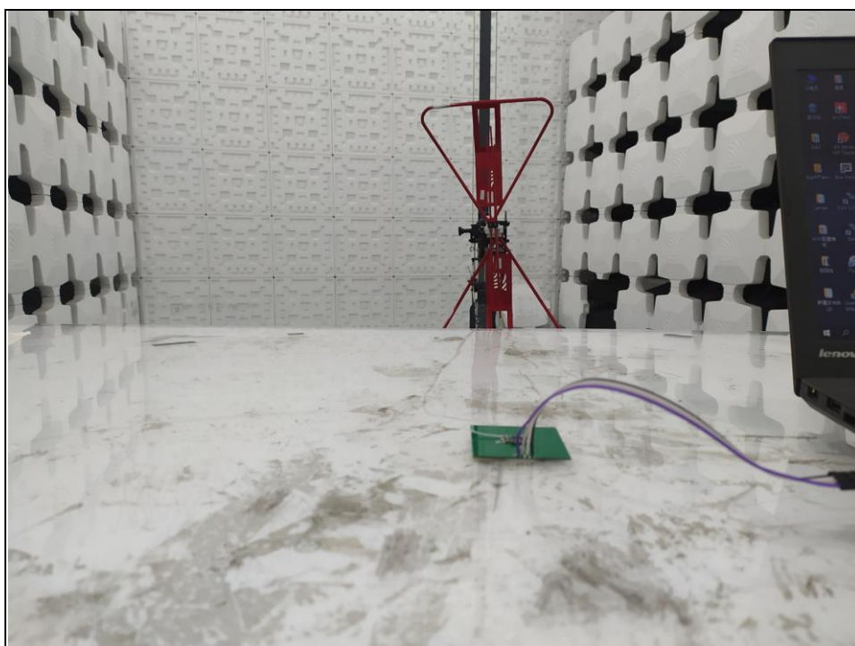
Radiated emission test: Frequency Range < 30MHz ~1GHz >
