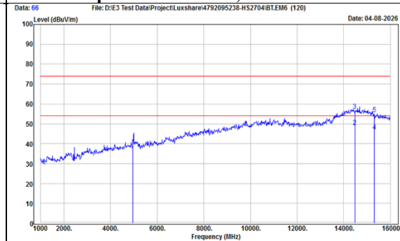
TX, 8DPSK - Emission (Ch 78) Radiated Spurious Emission, Vertical
