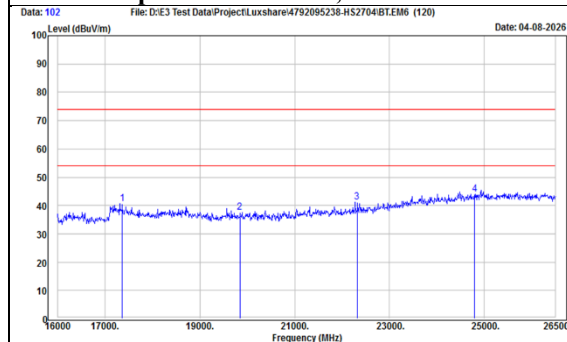
TX, 8DPSK - Emission (Ch 78) Radiated Spurious Emission, Horizontal
