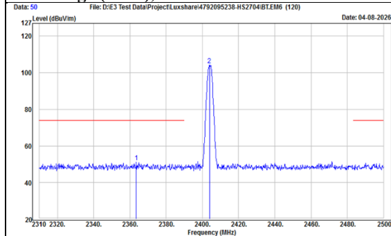
TX, BT-LE-2Mbps (Ch 1) Band Edge (Peak), Horizontal
