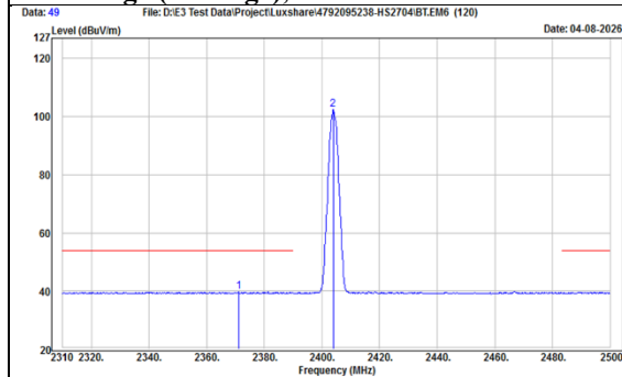
TX, BT-LE-2Mbps (Ch 1) Band Edge (Peak), Horizontal
