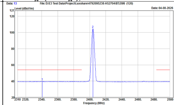
TX, BT-LE-2Mbps (Ch 1) Band Edge (Peak), Vertical
