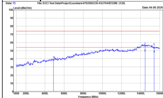
TX, BT-LE-2Mbps - Emission (Ch 19) Radiated Spurious Emission, Horizontal
