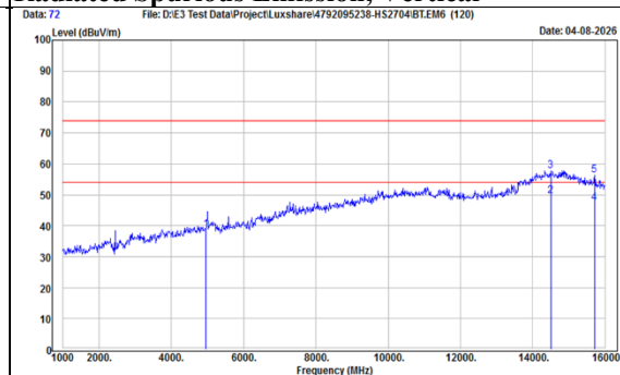
TX, BT-LE-1Mbps - Emission (Ch 39) Radiated Spurious Emission, Vertical
