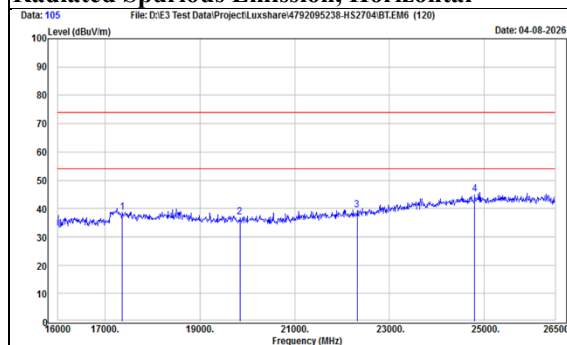
TX, BT-LE-1Mbps - Emission (Ch 39) Radiated Spurious Emission, Horizontal
