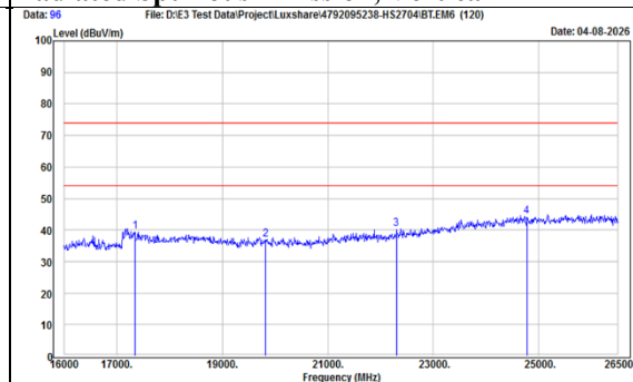
TX, BT-LE-2Mbps - Emission (Ch 38) Radiated Spurious Emission, Vertical
