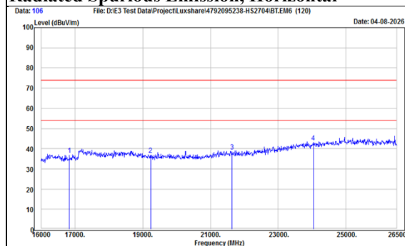
TX, BT-LE-2Mbps - Emission (Ch 1) Radiated Spurious Emission, Horizontal
