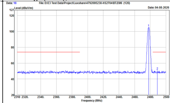
TX, BT-LE-2Mbps (Ch 38) Band Edge (Peak), Vertical
