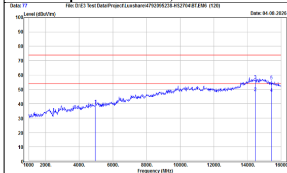
TX, BT-LE-2Mbps - Emission (Ch 38) Radiated Spurious Emission, Horizontal
