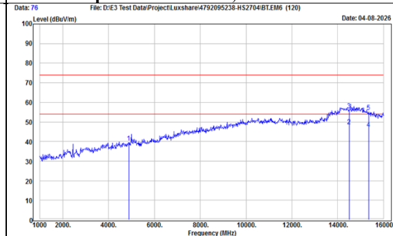
TX, BT-LE-2Mbps - Emission (Ch 19) Radiated Spurious Emission, Vertical
