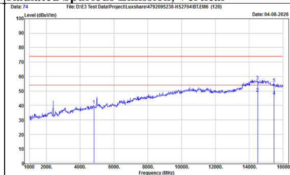
TX, BT-LE-2Mbps - Emission (Ch 1) Radiated Spurious Emission, Vertical
