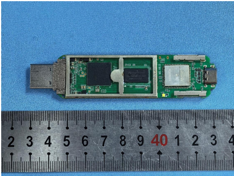
Sample 3: eMMC: FEMDNN008G-C9X08 and DDR: RS512M16ZSDD-75DT
