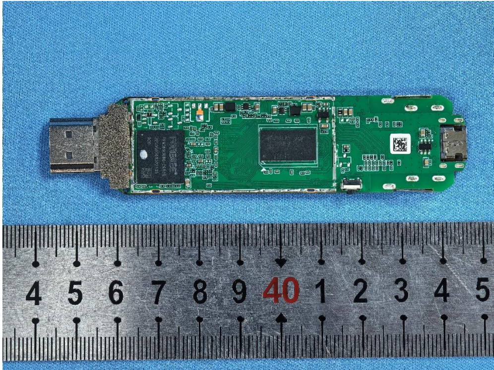
Sample 1: eMMC: FEMDNN008G-C9A39 and DDR: MT40A512M16LY-062E:E
