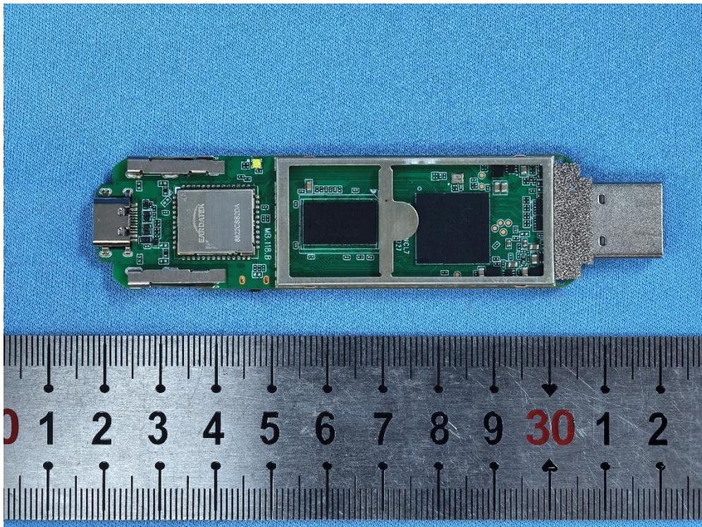
Sample 2: eMMC: FEMDNN008G-C9A39 and DDR: BWND4X16I8B-8Gb
