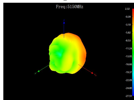
ZXY face @5150MHz
