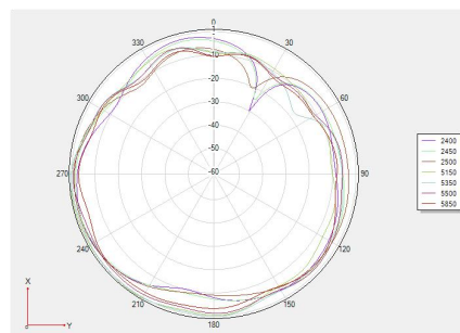
Theta =90 freq=2400MHz
