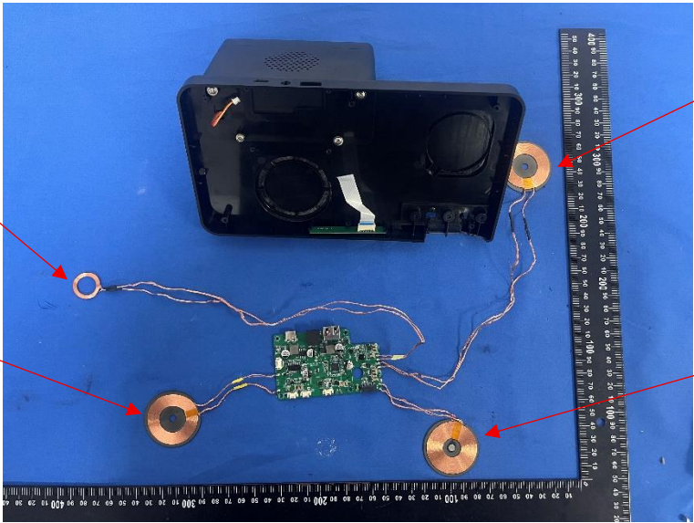
Loop Coil Antenna 1
