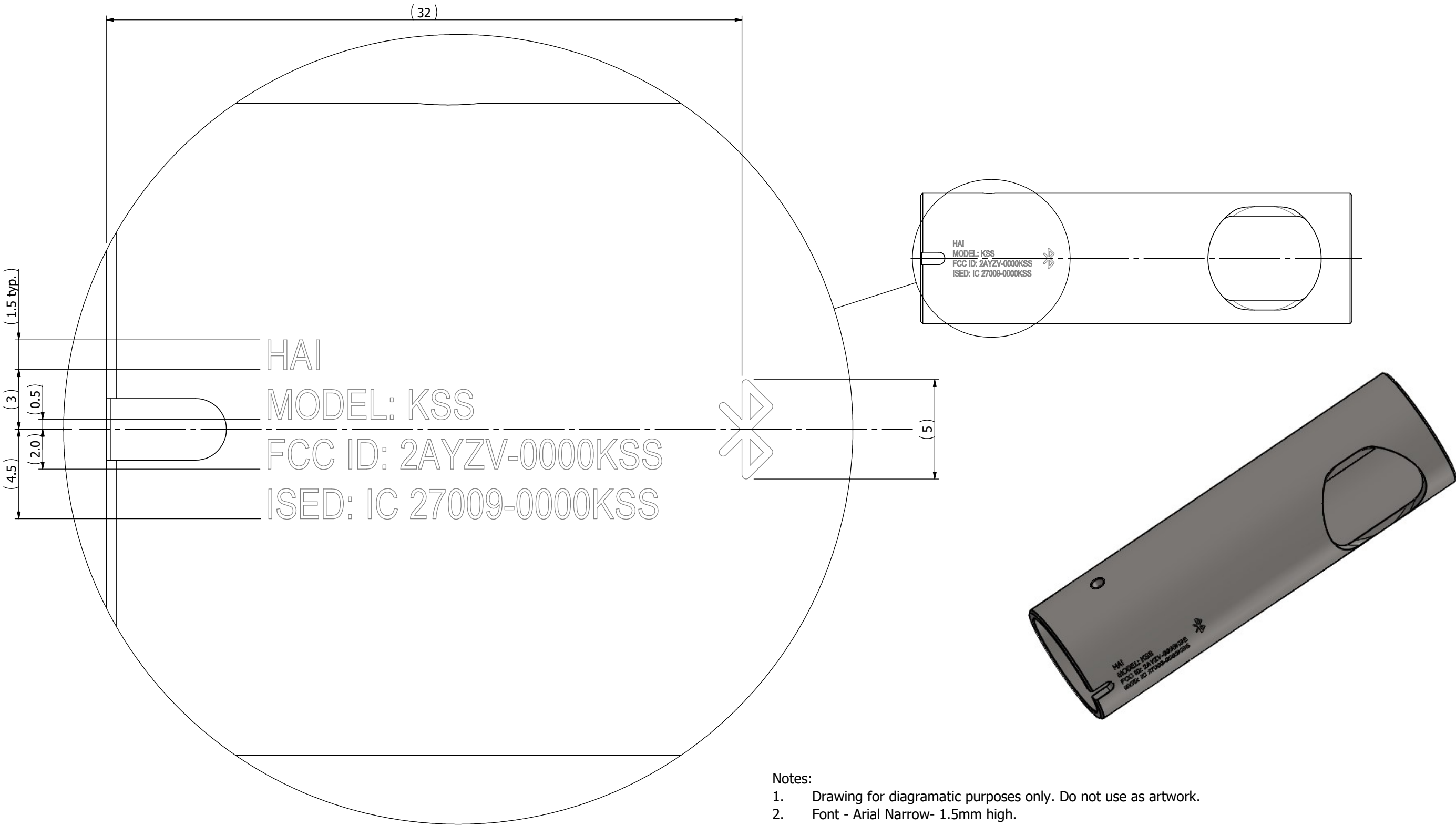
DETAIL E SCALE 5 : 1
