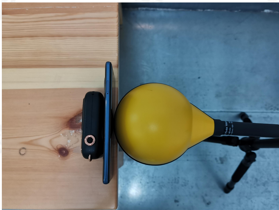
The worst test setup photo: top 0cm
