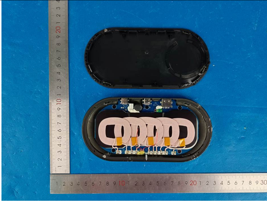
Photo 1 (For model ZDWCSW5)
