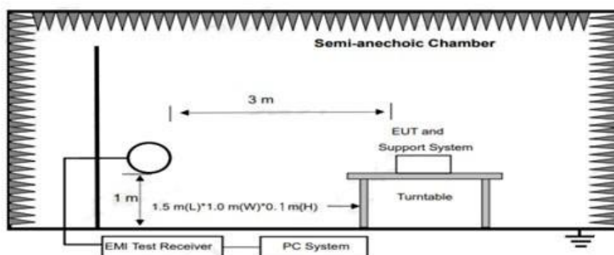
Test set-up of radiated disturbance (below 30MHz)
