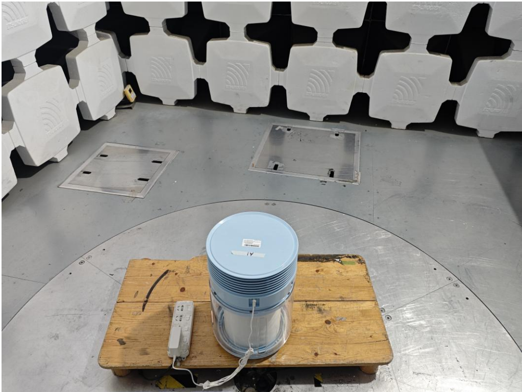
(The EUT was placed in the center of the turntable)
