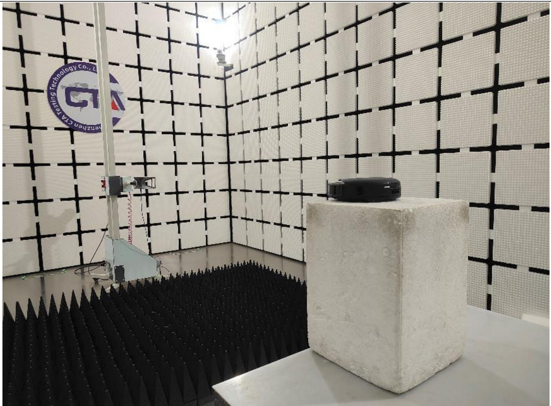
Emissions in frequency bands (above 1GHz)
