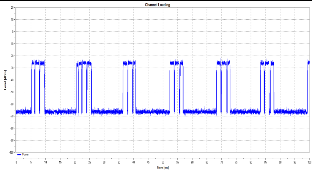
11N20SISO_5500
