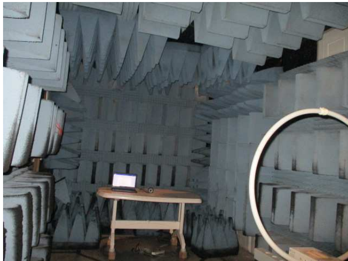
Figure 5. Radiated Emission Test, 0.009-30MHz
