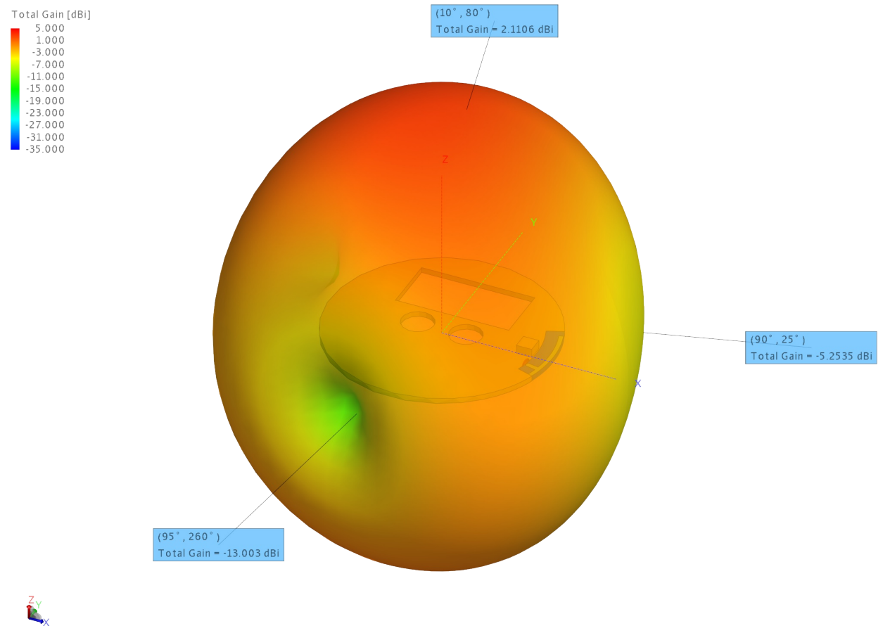
Figure 5: 3D View
