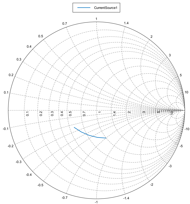
Figure 3: Impedance - VC3_R8_optimum
