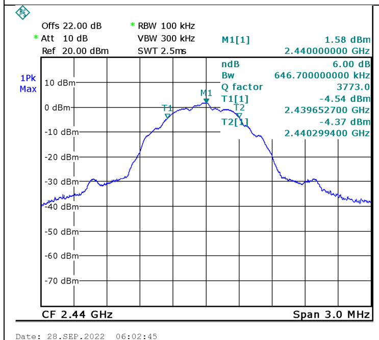
Figure 11. 2440.0 MHz, BLE
