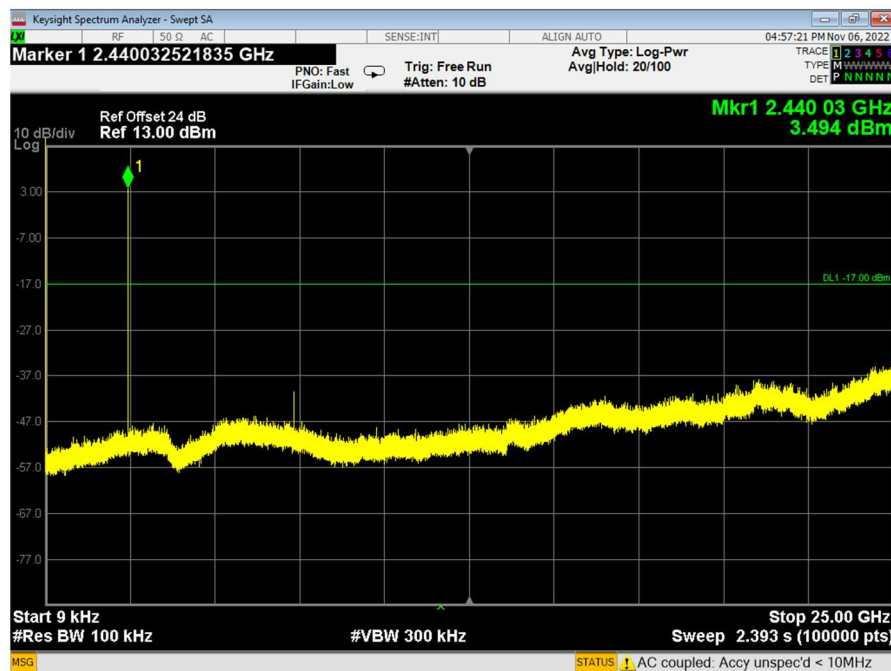
Figure 34 2440.0 MHz, BLE
