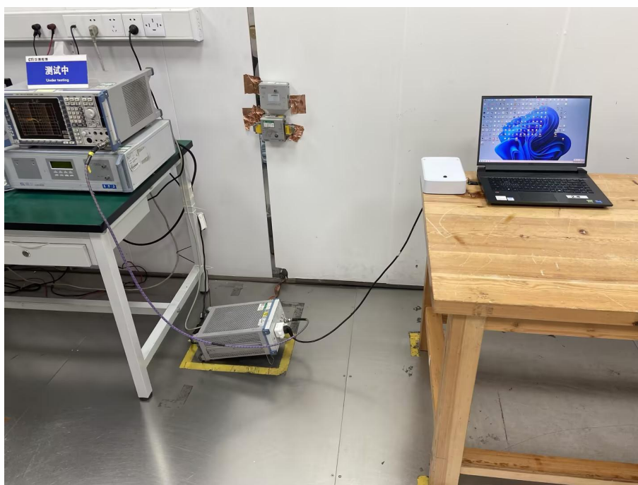
AC Power Line Conducted Emissions Test Setup-4
