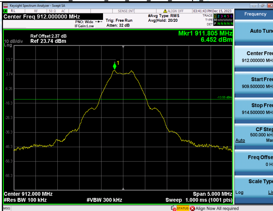
2_Bandedge_NVNT_ANT1_100Kbps_912
