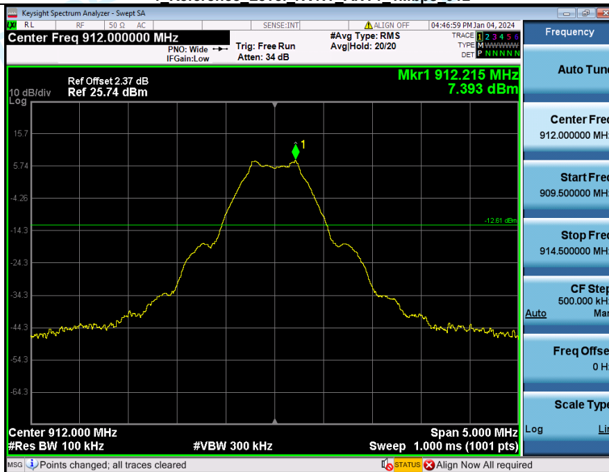
2 Spurious Emission NVNT ANT1 1Mbps 912
