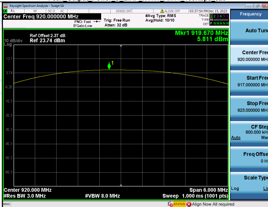
Peak Output Power & EIRP NVNT ANT1 100Kbps 920
