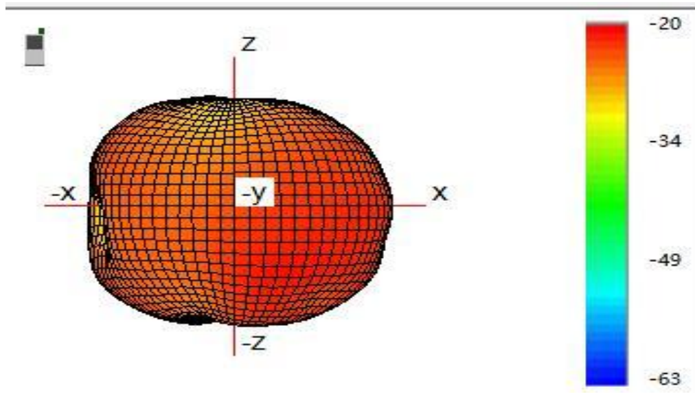
(4) Typical Free Space 3D Radiation Pattern at 914MHz(unit:dBi):
