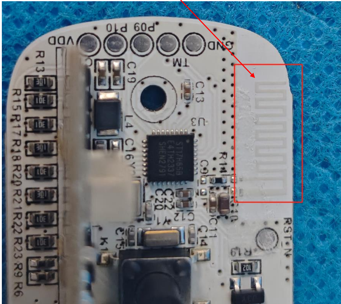
View of wireless antenna
