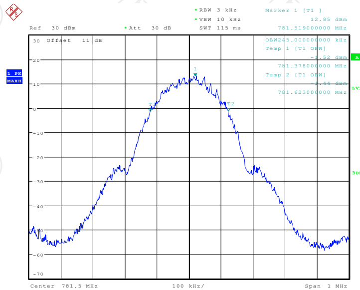
Band13 GSM UL output
