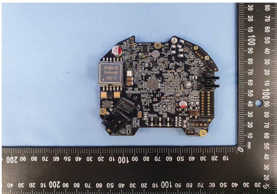
EUT Photo (42)
