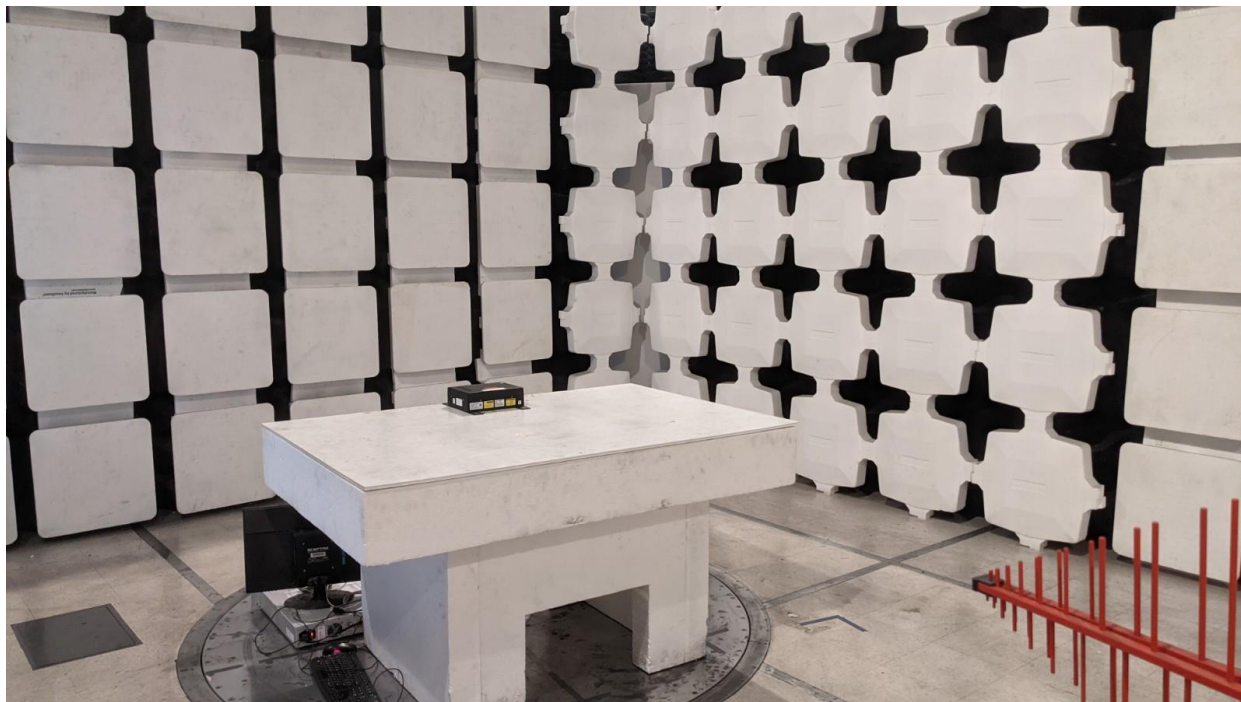
Digital Emissions 30M - 1GHz
