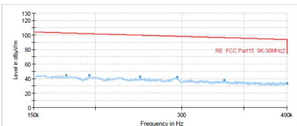
Radiates Emission from 150kHz to 490kHz
