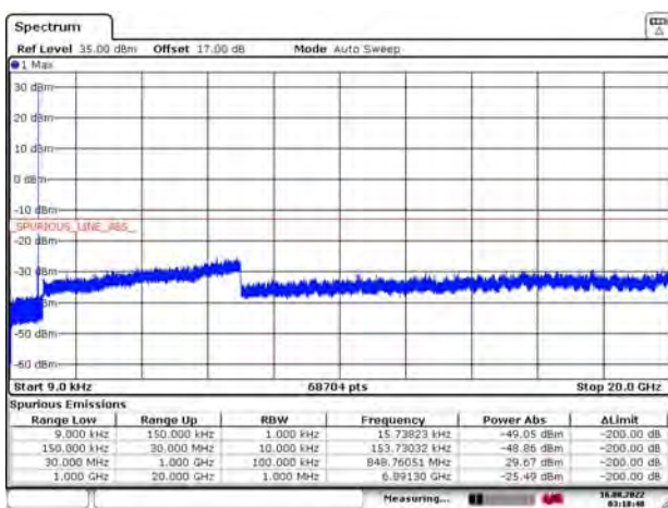
GPRS GSM 850 CH- High 9kHz ~ 20GHz
