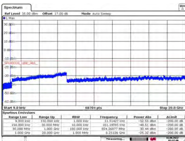
GPRS GSM 850 CH-Low 9kHz ~ 20GHz
