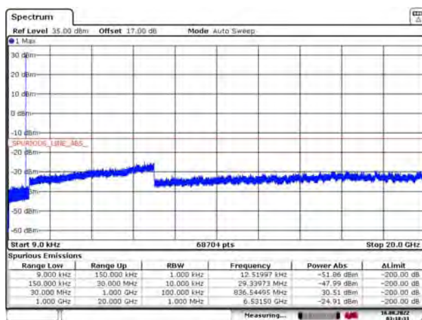
GPRS GSM 850 CH- Middle 9kHz ~ 20G
