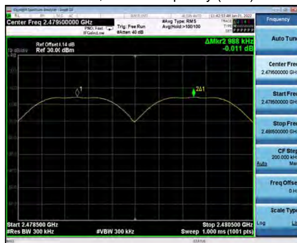
BT DH5 CH78, Carrier frequency (MHz): 2480
