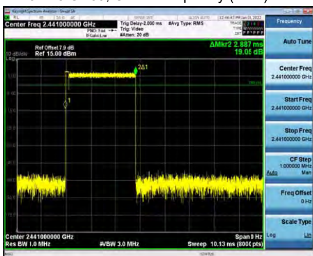
BT 3DH5 CH39, Carrier frequency (MHz): 2441
