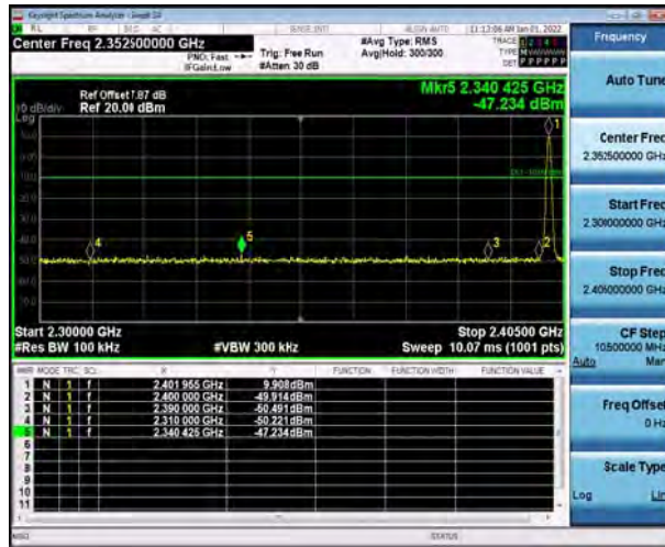
BT 2DH5 CH0, Carrier frequency (MHz): 2402
