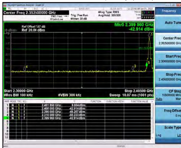
BT 3DH5 CH0, Carrier frequency (MHz): 2402
