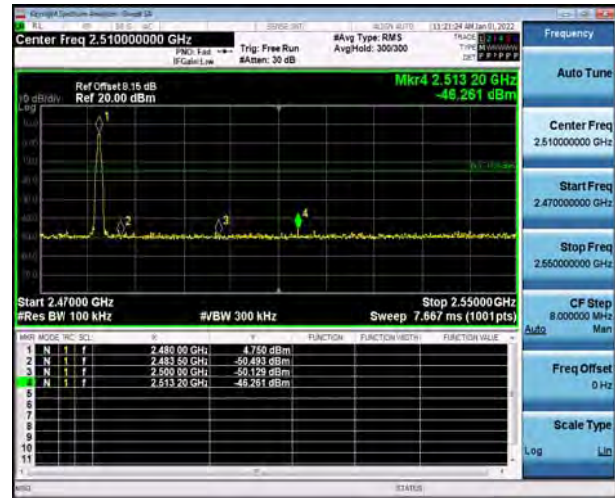
BT 2DH5 CH78, Carrier frequency (MHz): 2480
