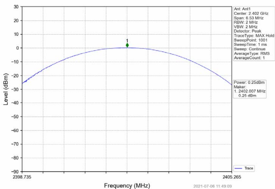
\pi /4-QPSK_2DH5_LCH_2402MHz_Ant1_NTNV
