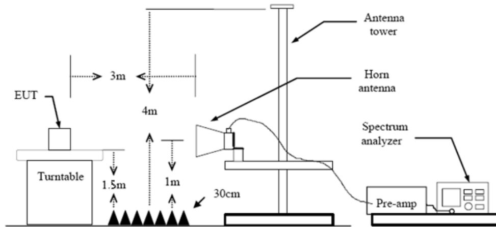
Above 1000MHz Test Setup
