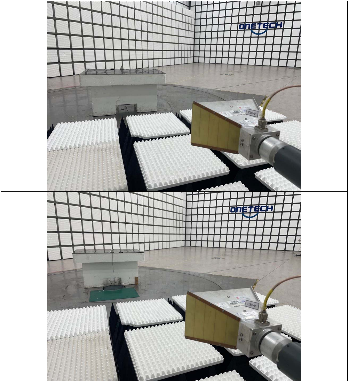
Radiated Disturbance Test Set Up (Above 1 GHz)
