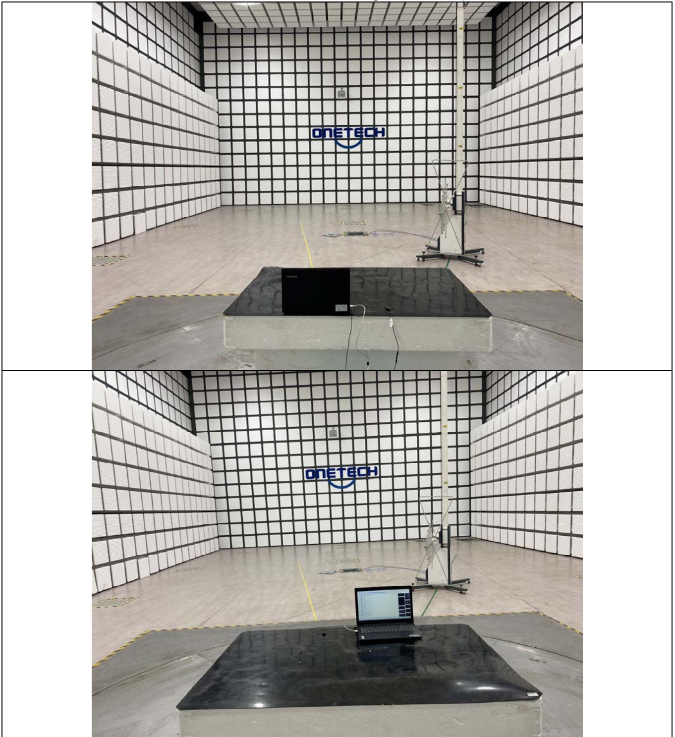
Radiated Emission Test Set Up (Below 1 GHz)
