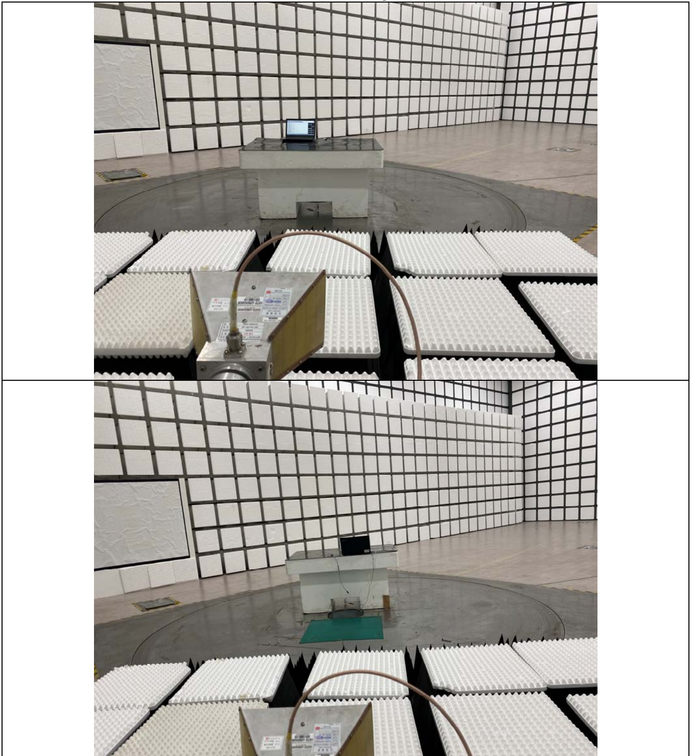
Radiated Emission Test Set Up (Above 1 GHz)
