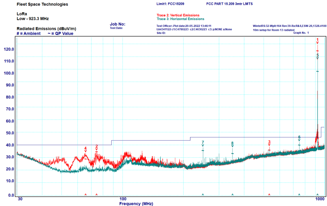
Graph 6-7: Transmitter Spurious Emissions, 30 – 1000 MHz, 923.3 MHz
