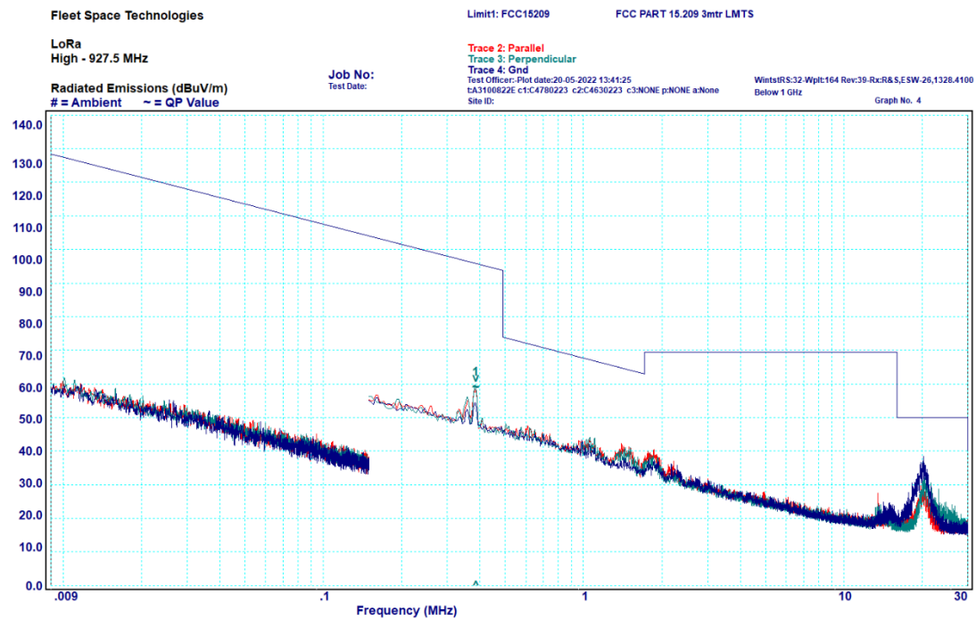
Graph 6-6: Transmitter Spurious Emissions, 9 kHz – 30 MHz, 927.5 MHz
