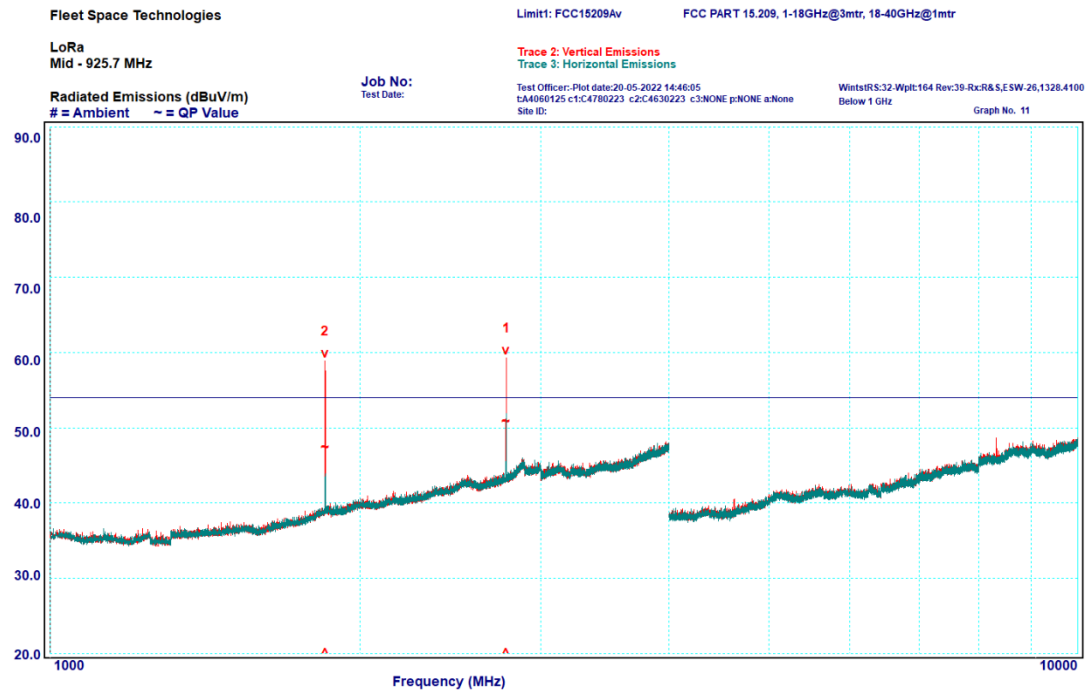
Graph 6-14: Transmitter Spurious Emissions, 1 – 10 GHz, Average, 925.7 MHz
