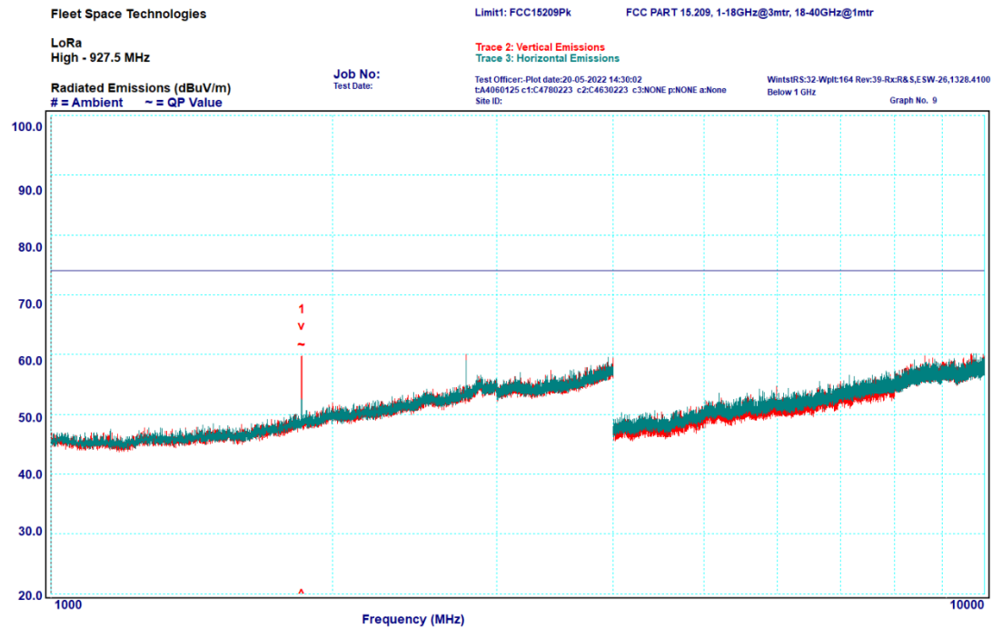
Graph 6-12: Transmitter Spurious Emissions, 1 – 10 GHz, Peak, 927.5 MHz
