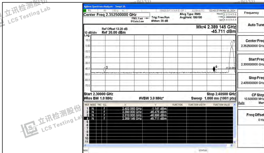
3DH5_Ant_Low_2402_Peak
