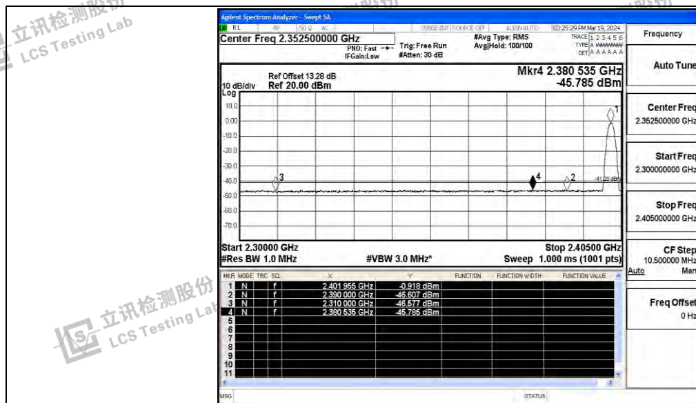
2DH5_Ant_Low_2402_Peak
