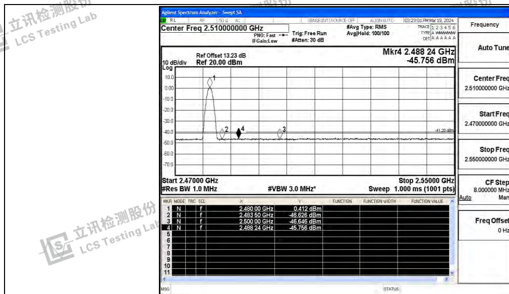
DH5_Ant_High_2480_Peak
