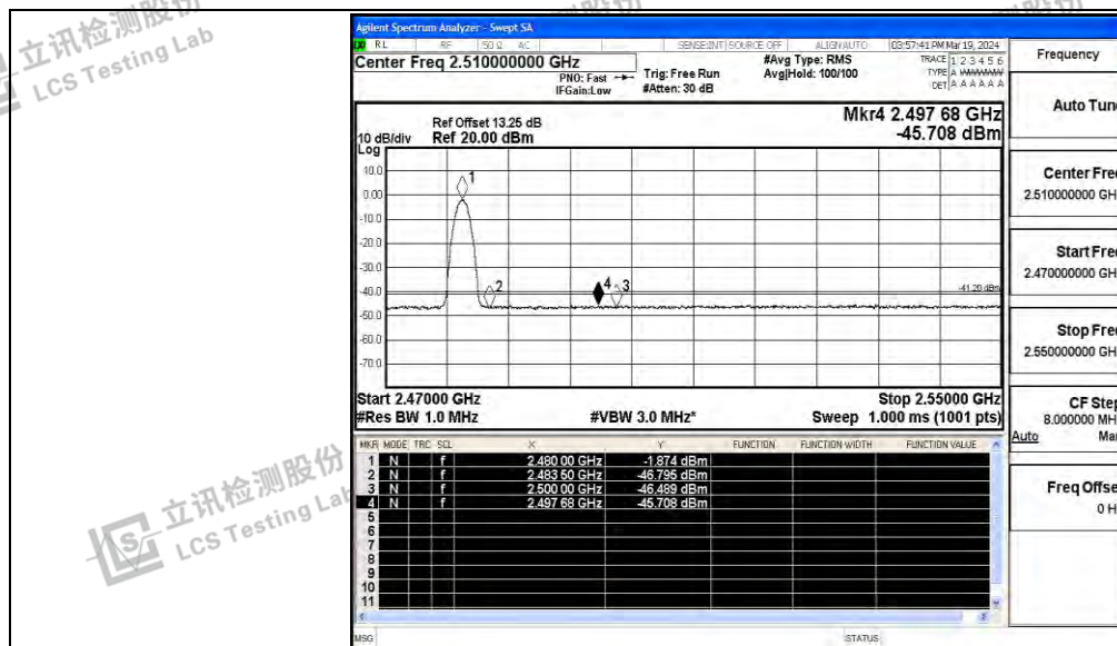
3DH5_Ant_High_2480_Peak
