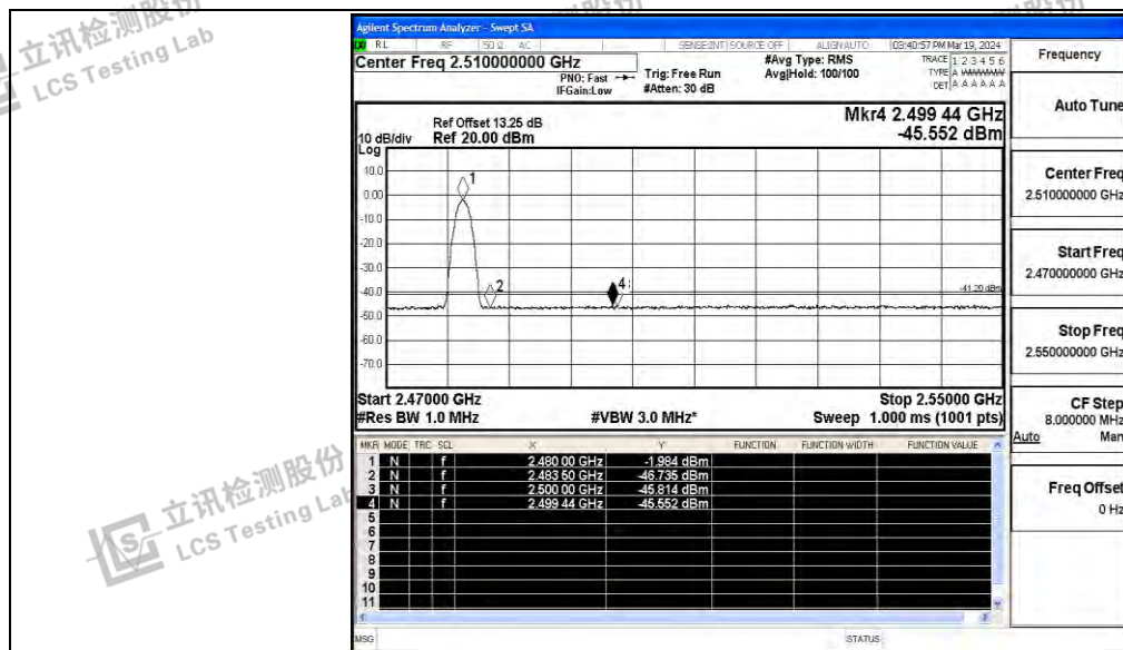
2DH5_Ant_High_2480_Peak
