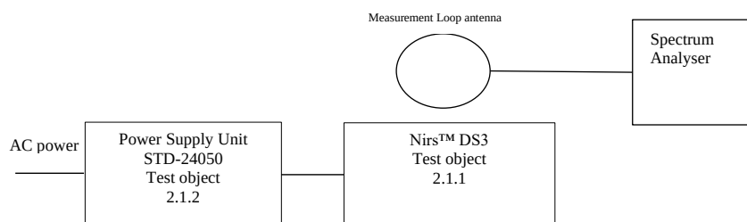
Figure 3.1.1 Block diagram of test objects with cables and auxiliary equipment, EMI test.
