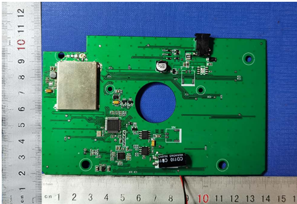
Photo 3
