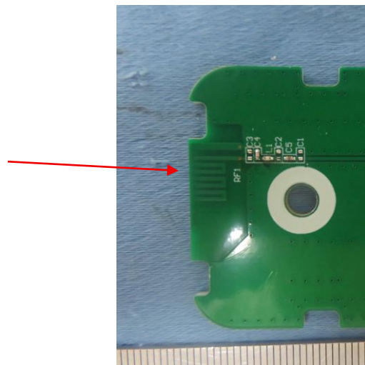
Antenna design:
