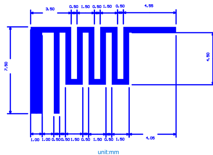
Antenna design:
