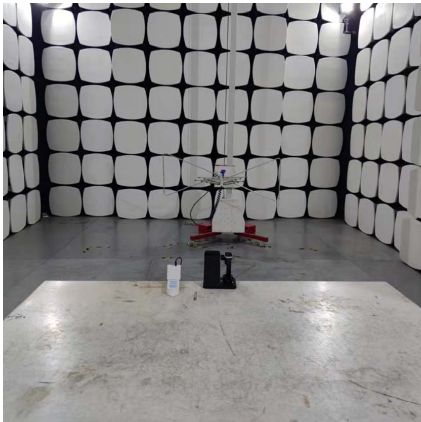
30MHz-1GHz
