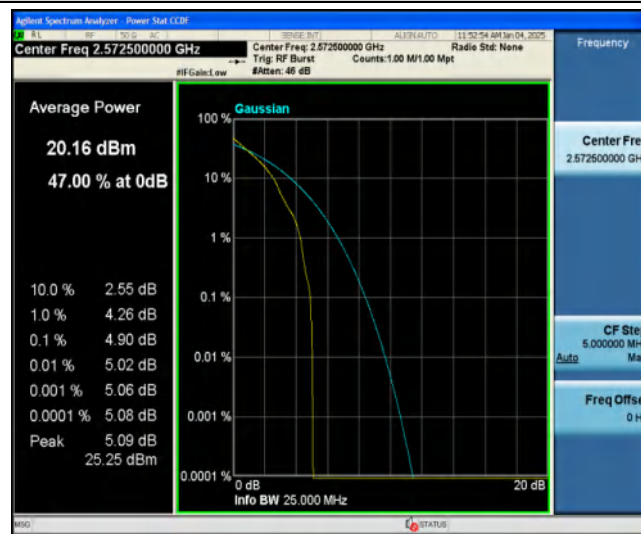
Band38-5MHz-QPSK-37775-25RB#0
