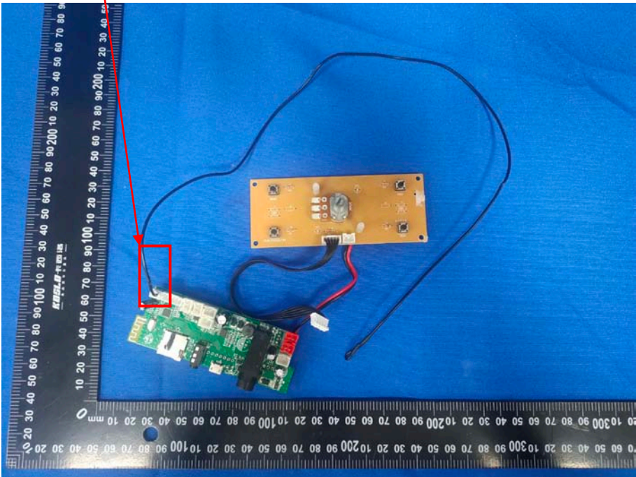
FM Antenna
