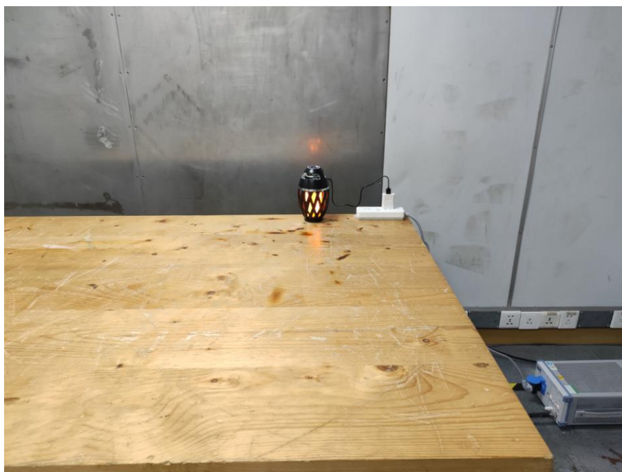
Photo of Power Line Conducted Emission Measurement
