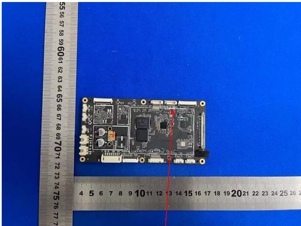
BT Antenna
